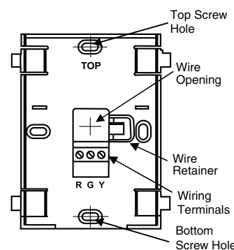
Figure C Front View of Back Plate
