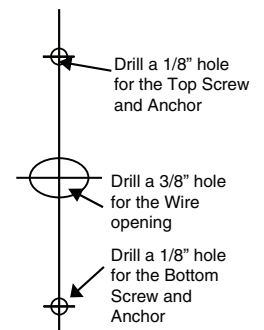
Figure D Drill holes in wall
